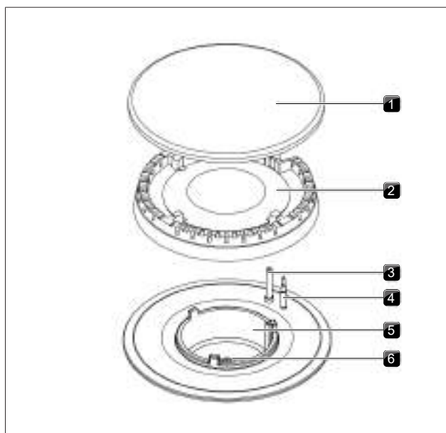
Fig. 4.48 Gas burner structure
