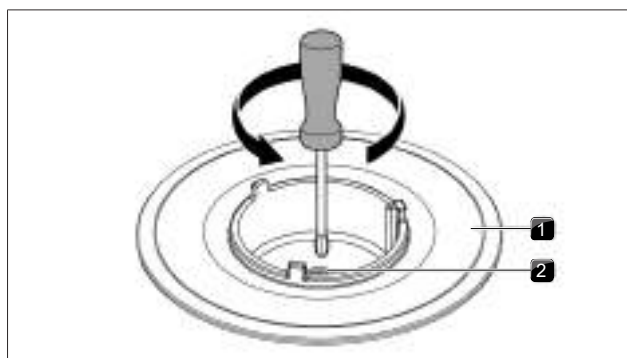
Fig. 4.49 Cooktop burner with gas burner nozzle
